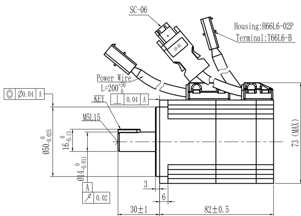
Mechanical View 3
