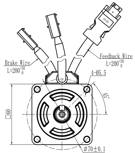
Mechanical View 2
