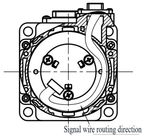
Mechanical View 8
