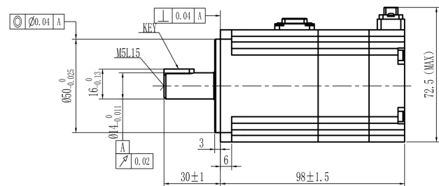
Mechanical View 9
