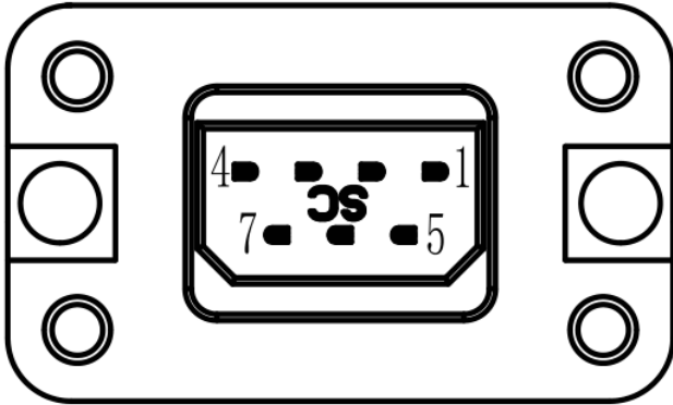
Mechanical View 3
