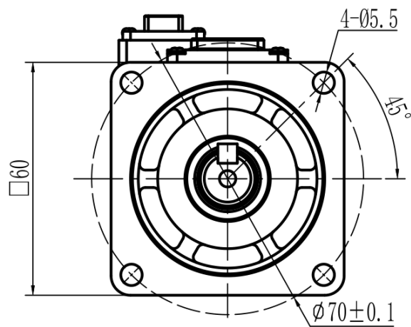
Mechanical View 10
