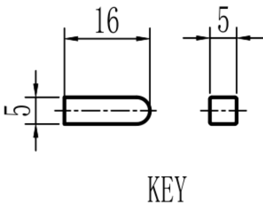
Mechanical View 5
