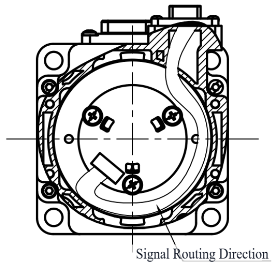
Mechanical View 7
