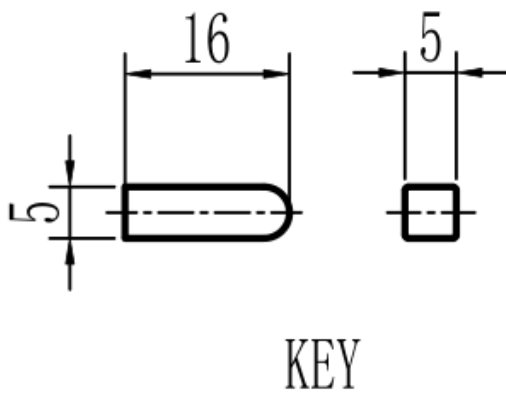
Mechanical View 6
