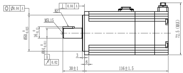
Mechanical View 10
