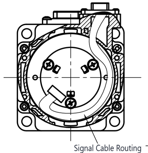
Mechanical View 8
