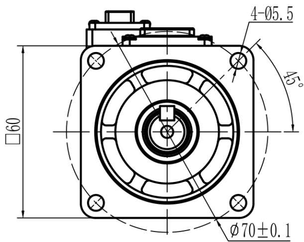
Mechanical View 9
