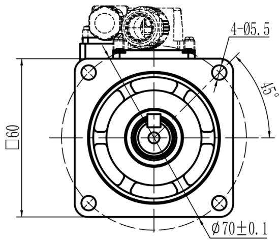
Mechanical View 8
