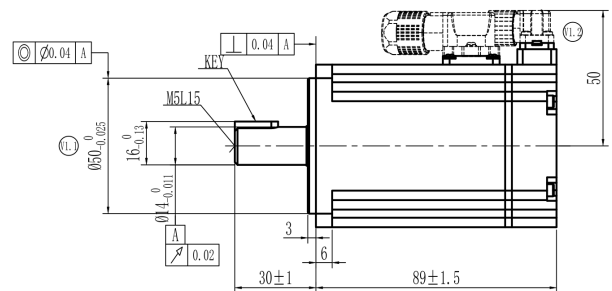
Mechanical View 7
