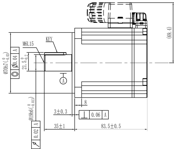
Mechanical View 3
