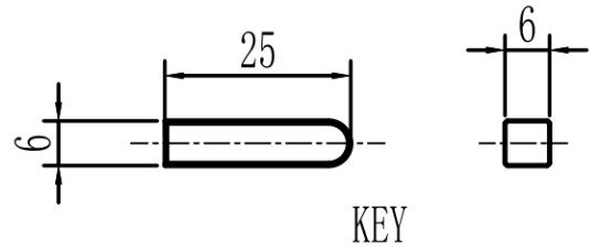
Mechanical View 2
