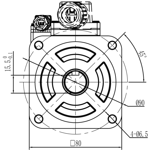
Mechanical View 1
