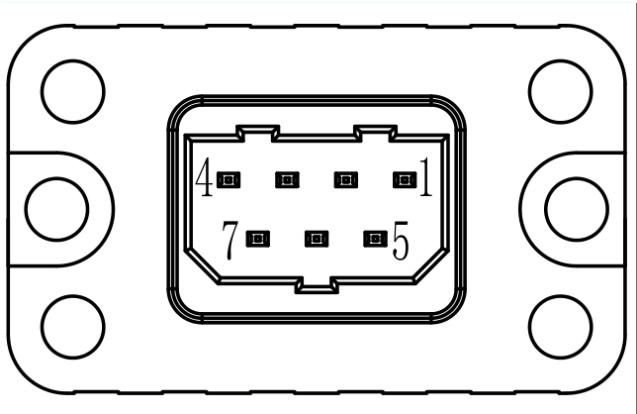
Mechanical View 6
