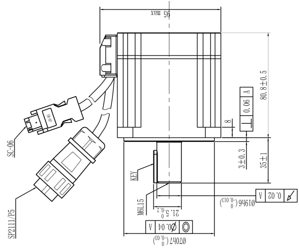
Mechanical View 2
