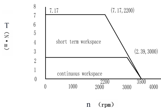
Mechanical View 9
