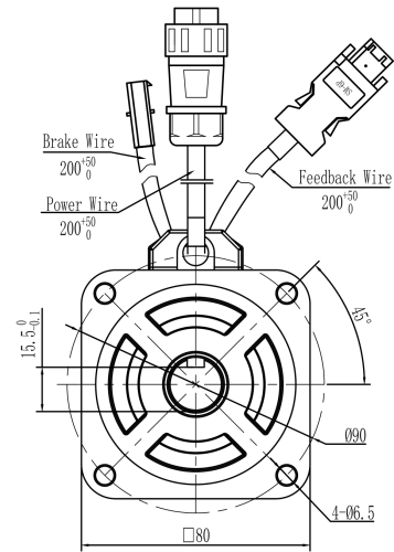
Mechanical View 2
