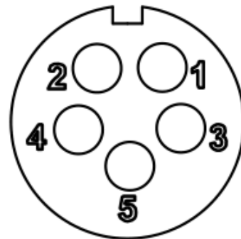
Mechanical View 2
