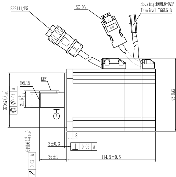
Mechanical View 1
