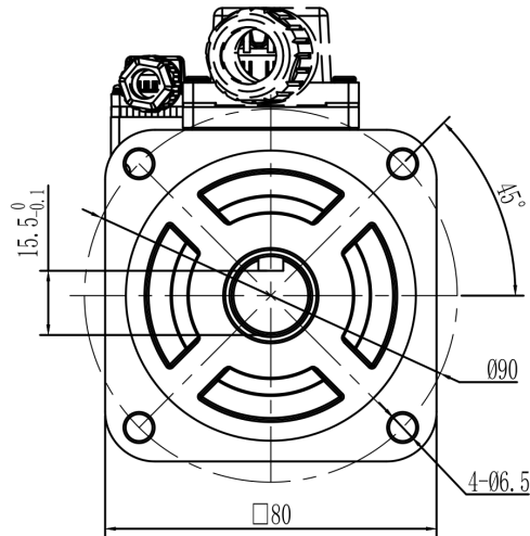
Mechanical View 1
