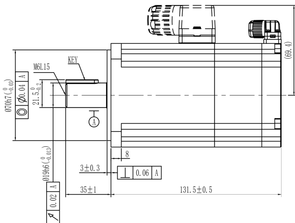
Mechanical View 3
