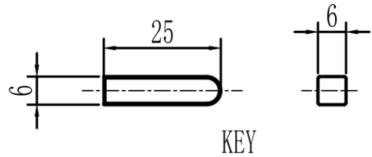
Mechanical View 2
