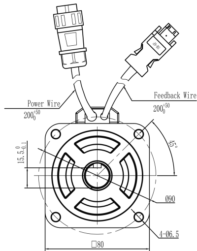
Mechanical View 1
