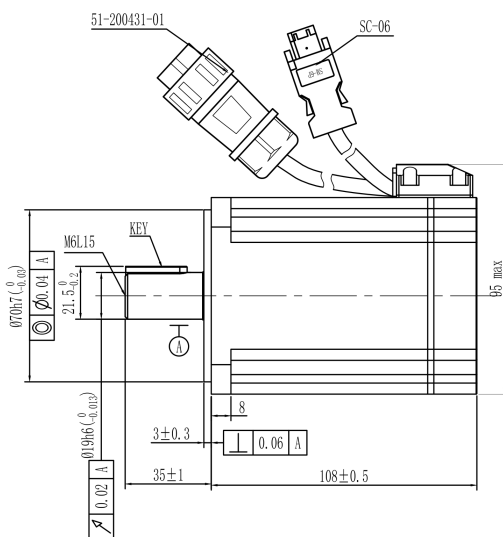
Mechanical View 3
