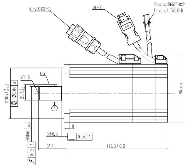
Mechanical View 2
