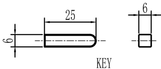
Mechanical View 3
