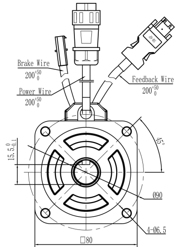
Mechanical View 2
