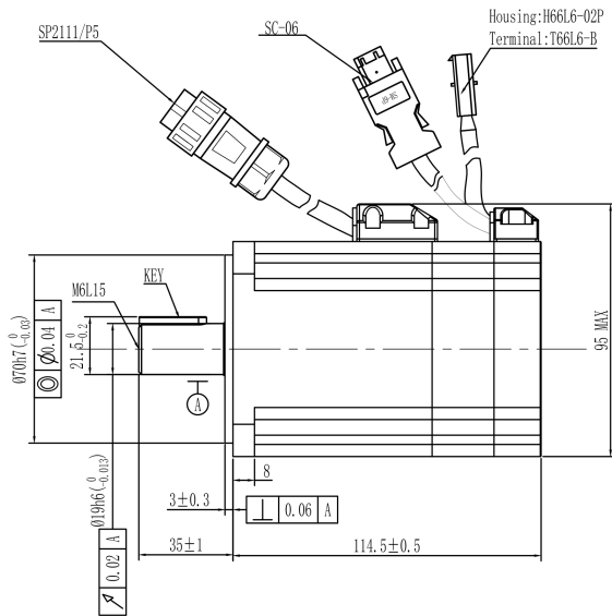
Mechanical View 1
