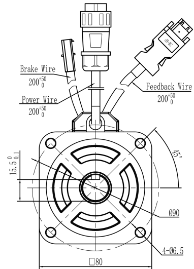
Mechanical View 2
