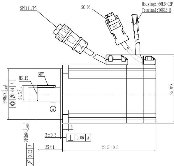
Mechanical View 1
