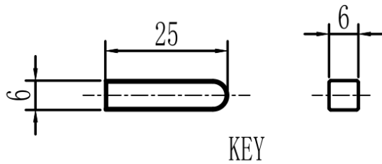
Mechanical View 3
