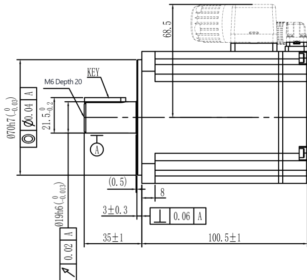
Mechanical View 8
