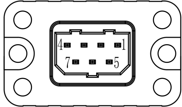
Mechanical View 4
