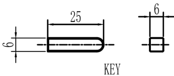
Mechanical View 5
