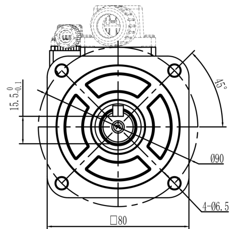
Mechanical View 6
