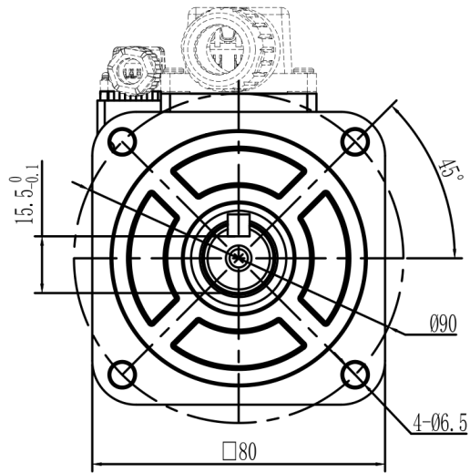
Mechanical View 8
