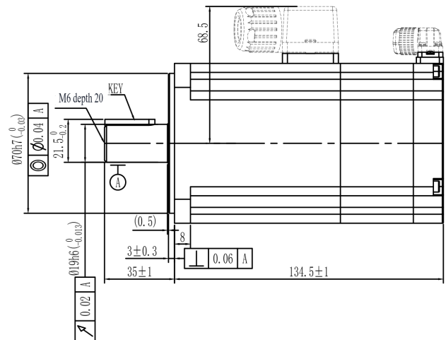
Mechanical View 7
