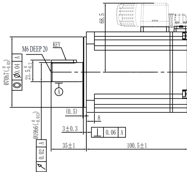
Mechanical View 7
