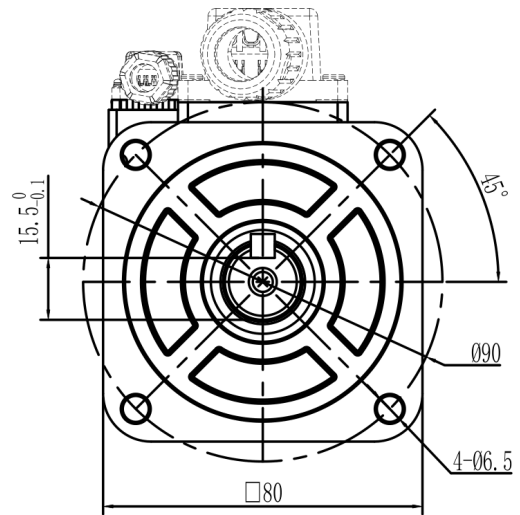
Mechanical View 9
