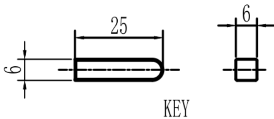
Mechanical View 7
