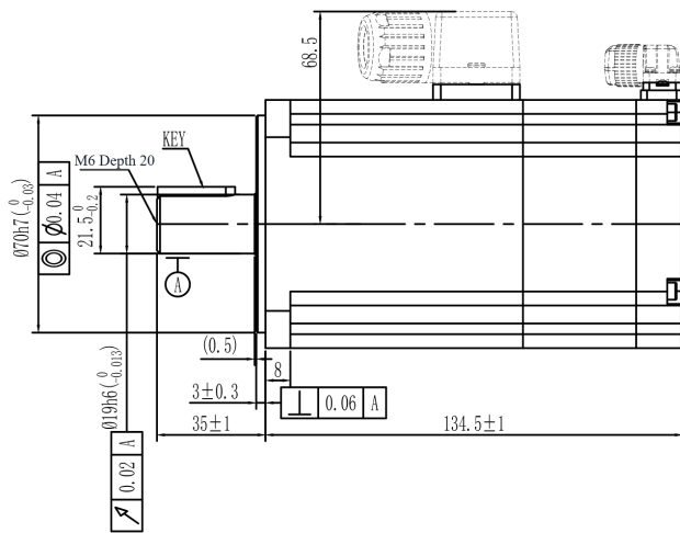
Mechanical View 9
