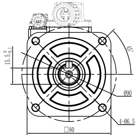
Mechanical View 8
