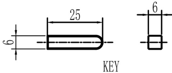
Mechanical View 6
