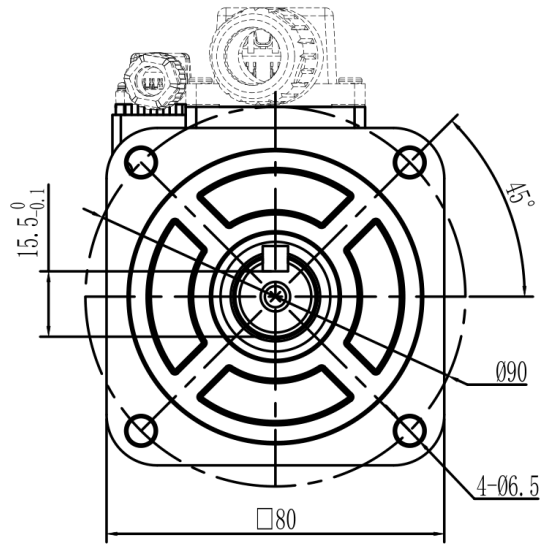
Mechanical View 8
