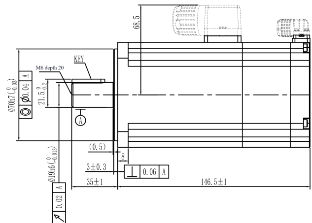
Mechanical View 7
