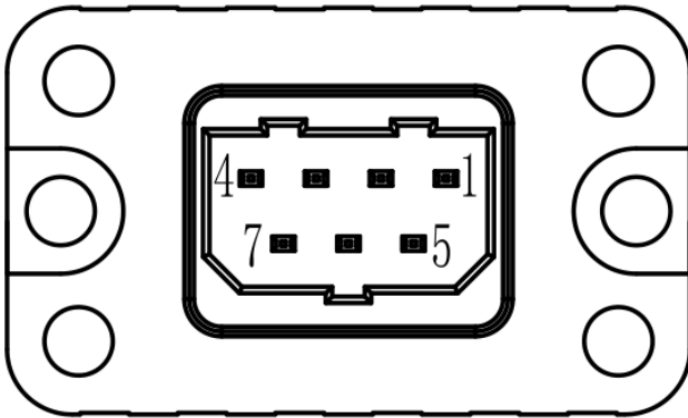
Mechanical View 3
