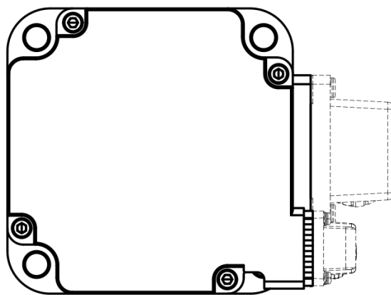
Mechanical View 9
