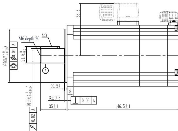
Mechanical View 8
