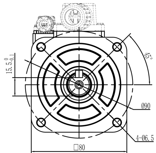
Mechanical View 7
