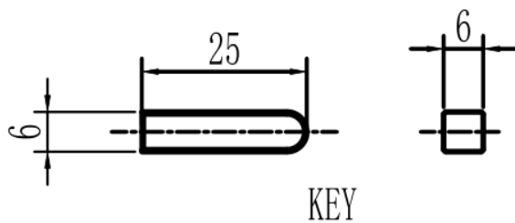
Mechanical View 6
