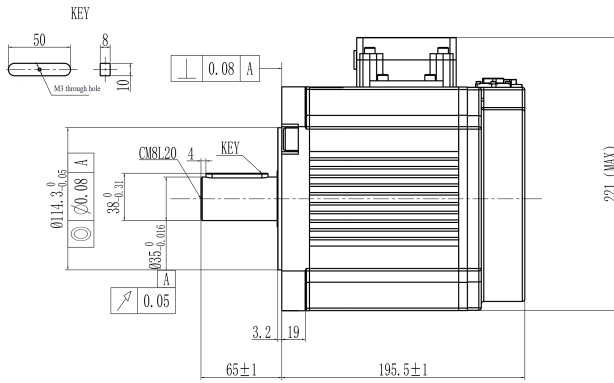
Mechanical View 1
