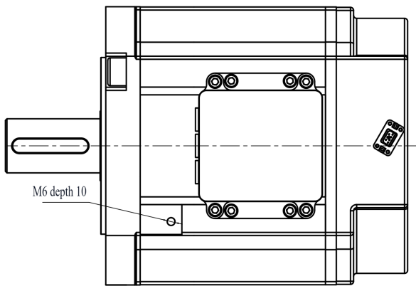
Mechanical View 3
