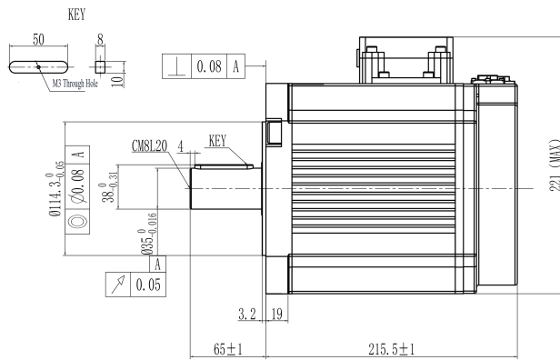
Mechanical View 1
