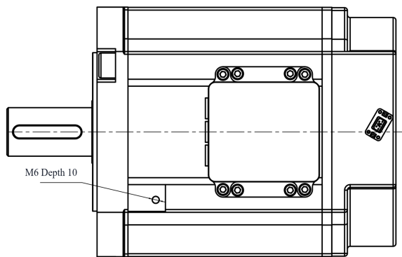
Mechanical View 3
