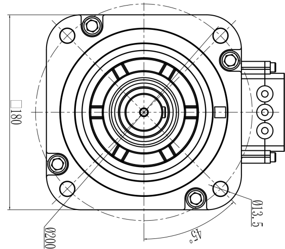
Mechanical View 2
