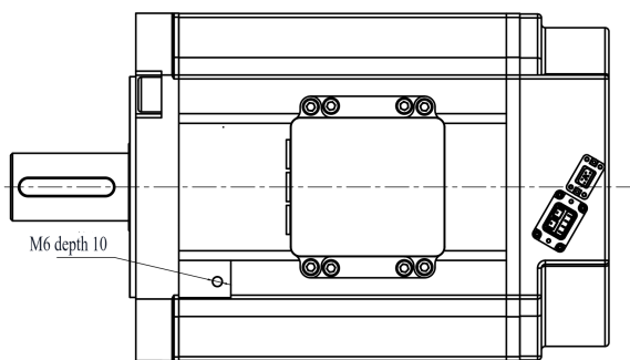
Mechanical View 3
