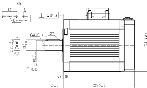
Mechanical View 1
