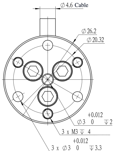
Mechanical View 1
