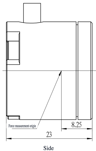
Mechanical View 1
