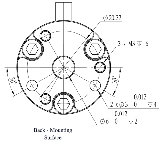
Mechanical View 2
