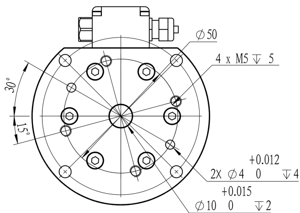
Mechanical View 3
