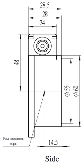
Mechanical View 1
