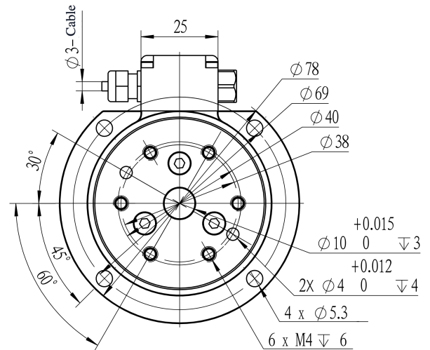
Mechanical View 2
