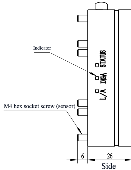
Mechanical View 3
