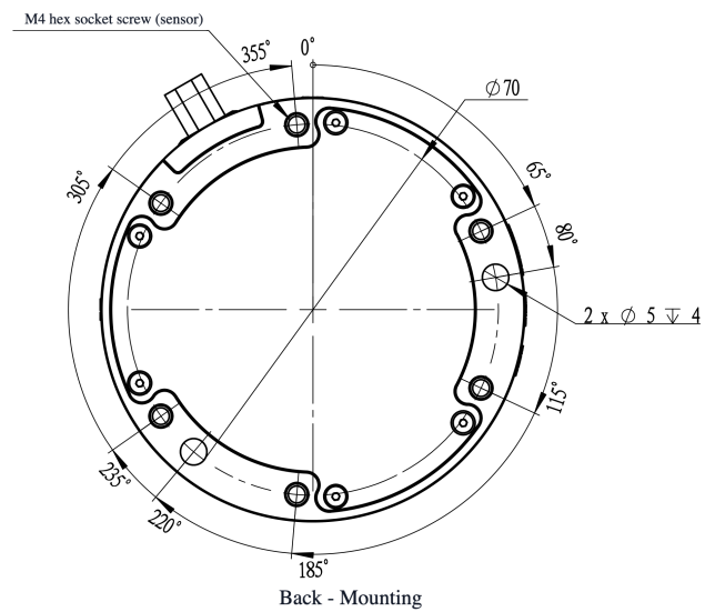
Mechanical View 2
