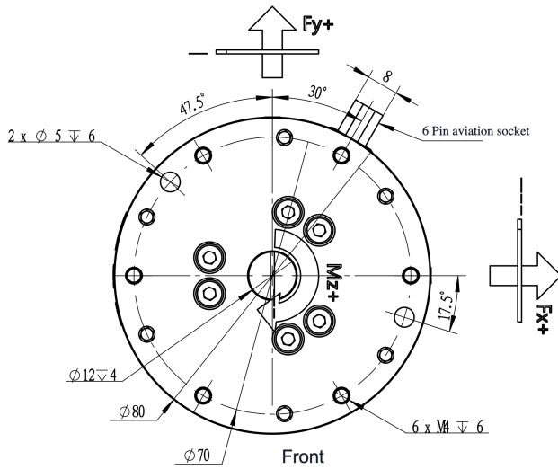
Mechanical View 1
