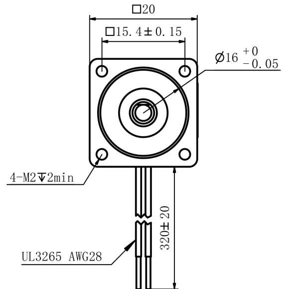
Mechanical View 2
