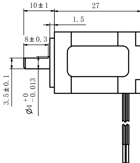
Mechanical View 1
