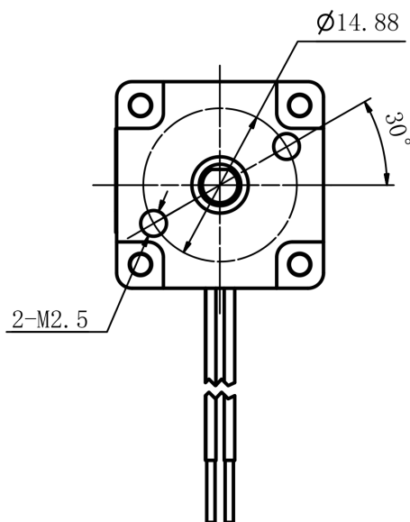
Mechanical View 3
