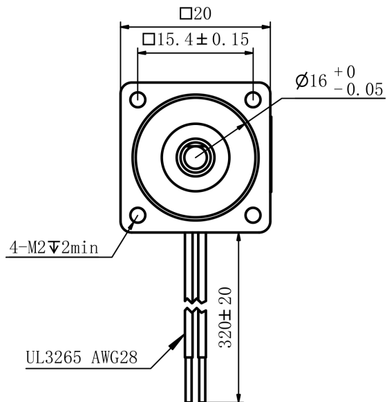
Mechanical View 1
