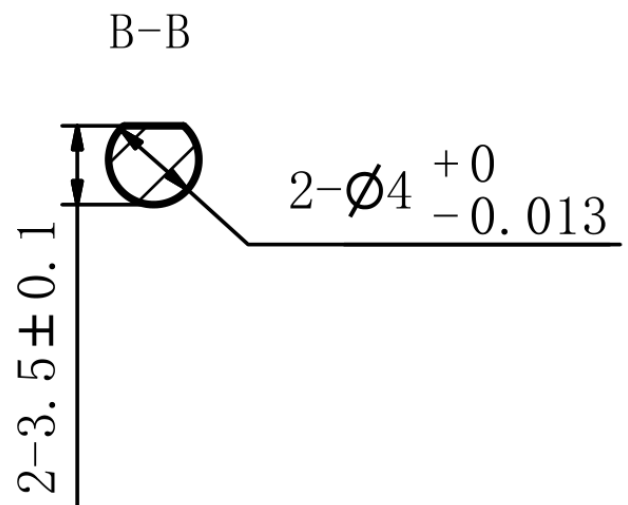
Mechanical View 4
