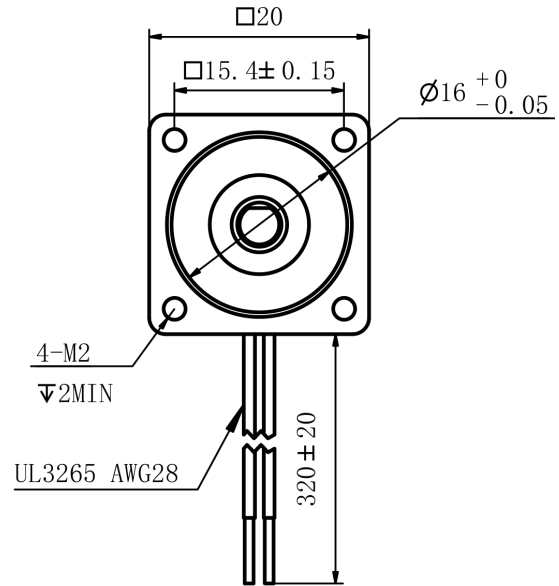
Mechanical View 2
