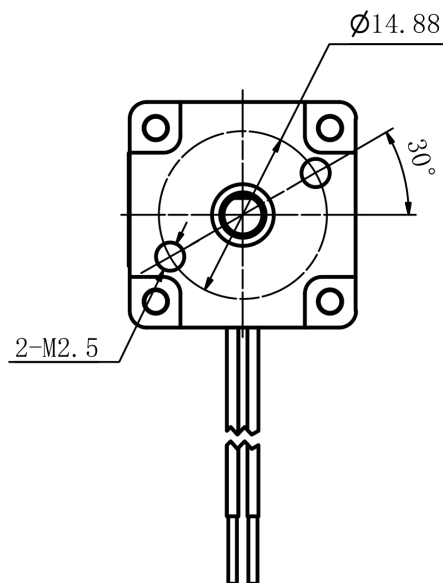
Mechanical View 3
