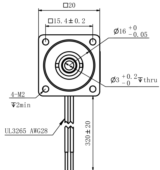
Mechanical View 2
