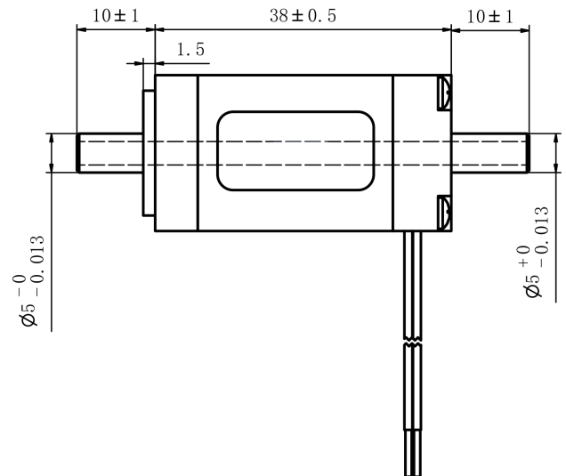
Mechanical View 2
