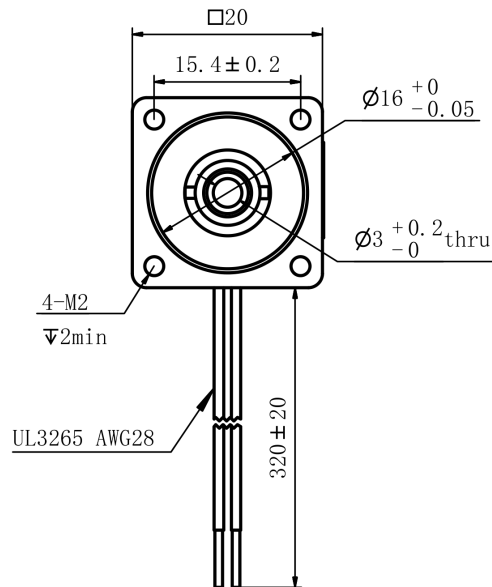
Mechanical View 1
