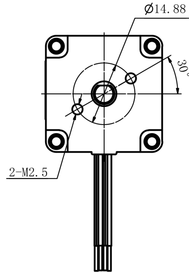
Mechanical View 2
