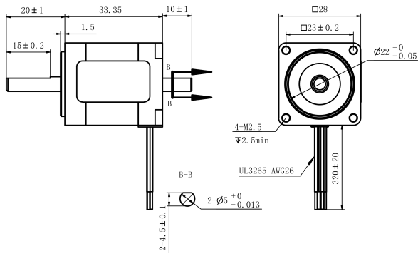
Mechanical View 1
