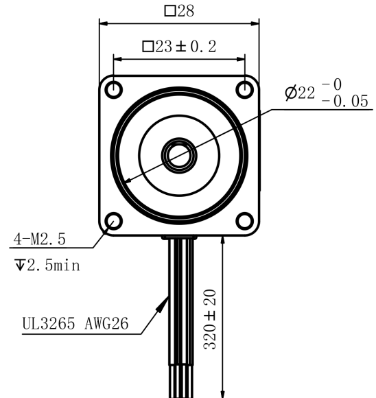
Mechanical View 2
