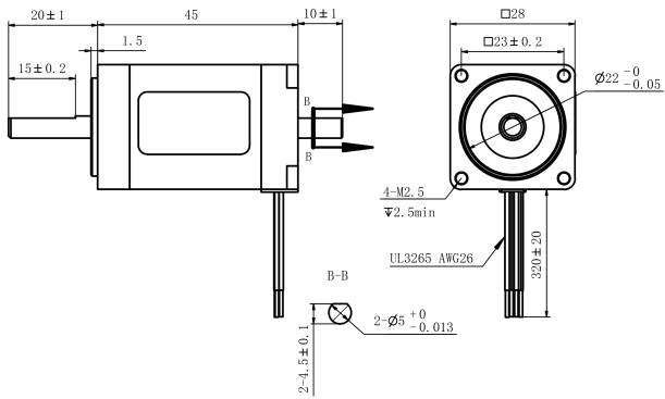
Mechanical View 1
