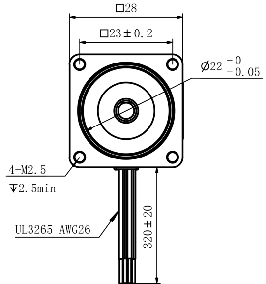
Mechanical View 2
