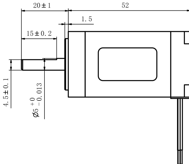
Mechanical View 1
