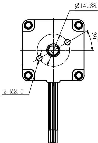
Mechanical View 3
