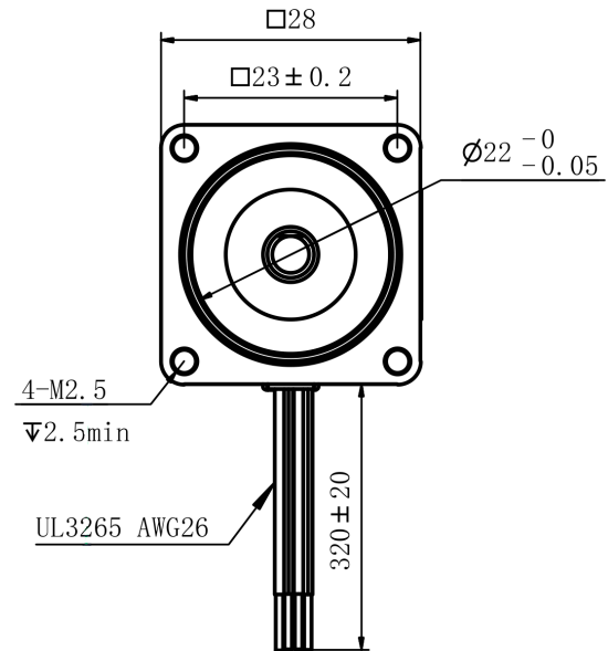
Mechanical View 2
