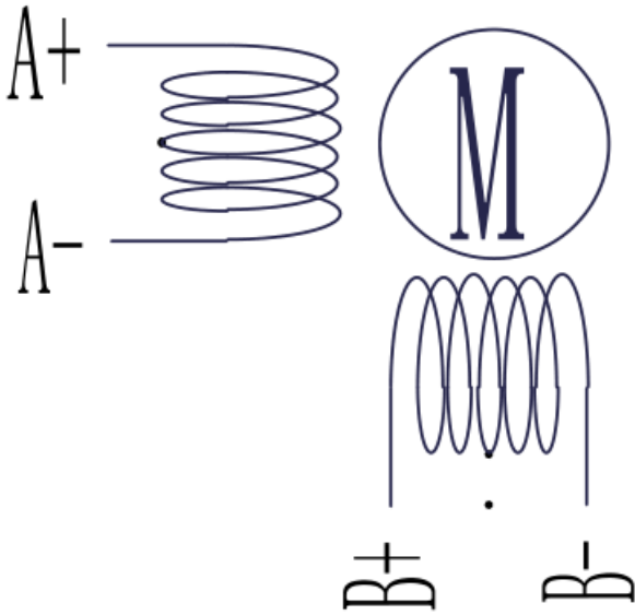
Mechanical View 8
