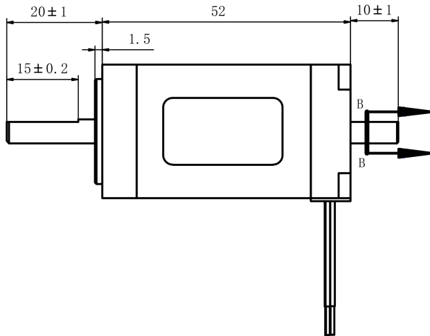
Mechanical View 1
