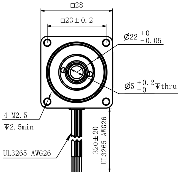
Mechanical View 1
