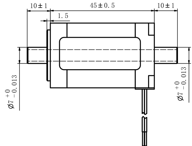
Mechanical View 2
