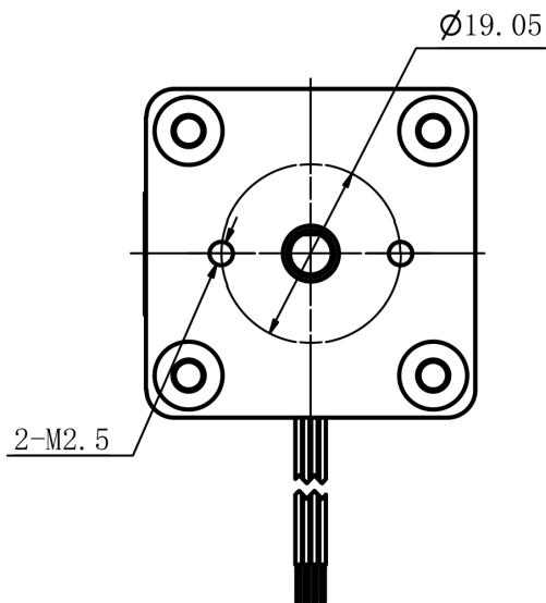
Mechanical View 3
