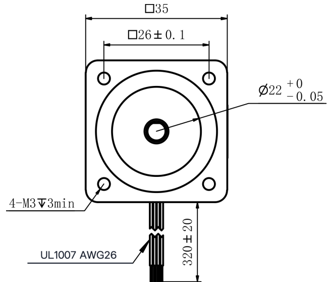
Mechanical View 2
