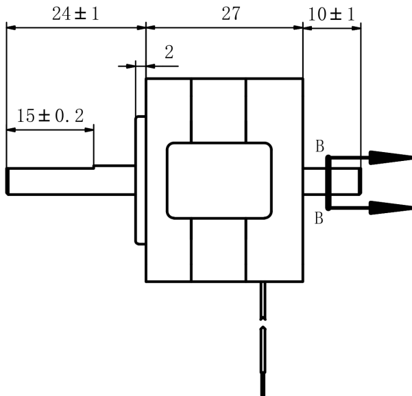
Mechanical View 1
