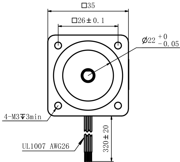
Mechanical View 1
