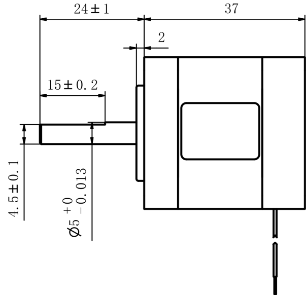
Mechanical View 2
