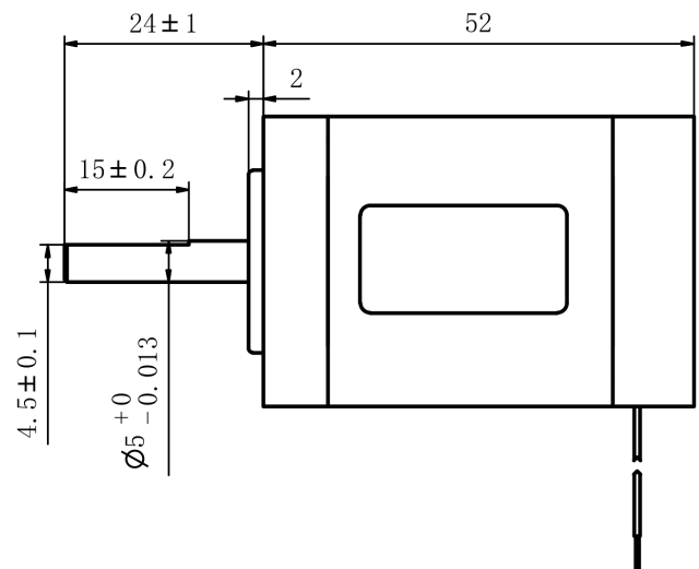
Mechanical View 2
