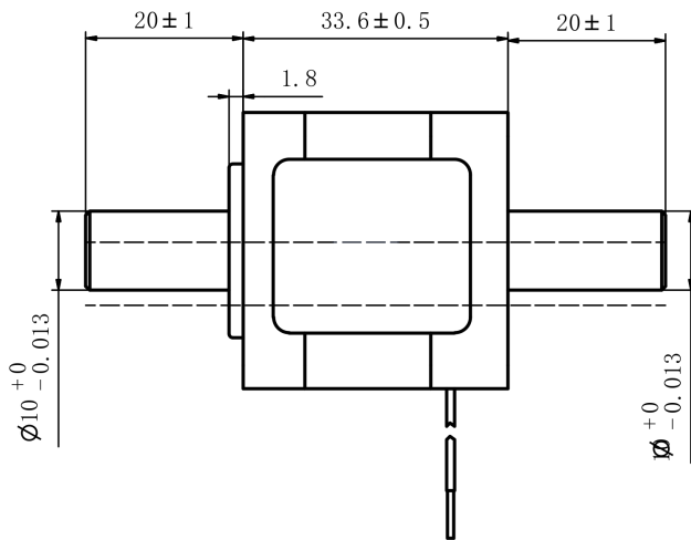
Mechanical View 1
