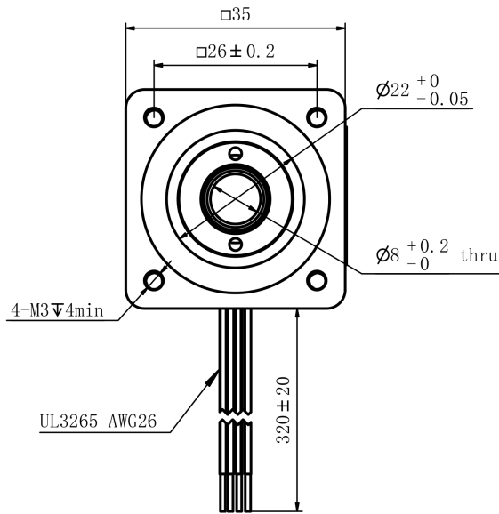
Mechanical View 1
