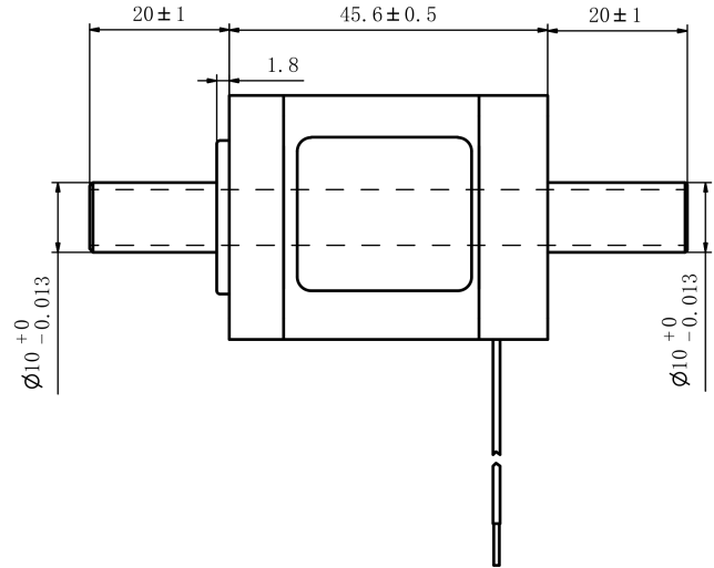
Mechanical View 2
