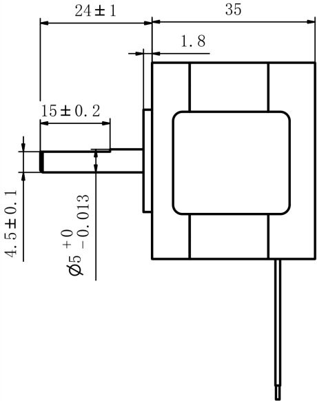
Mechanical View 2
