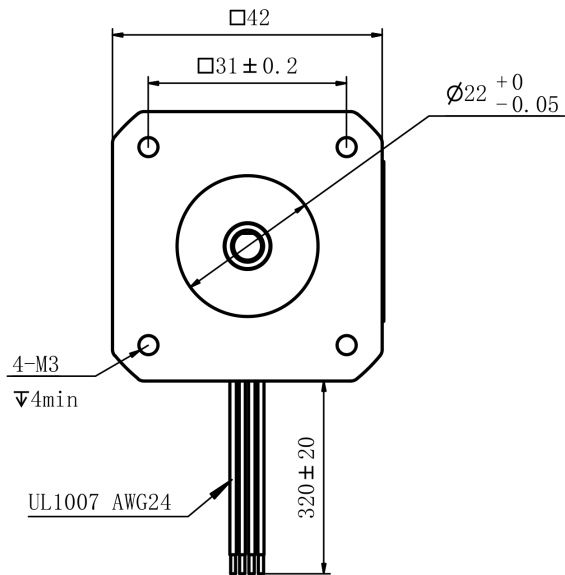
Mechanical View 1
