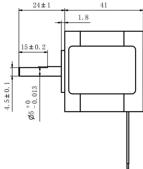
Mechanical View 2
