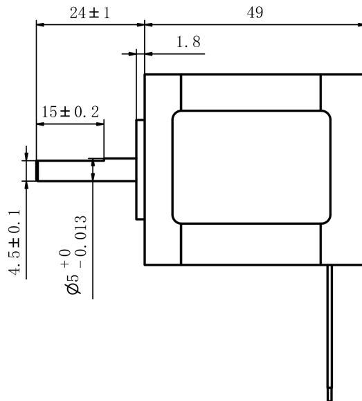
Mechanical View 1
