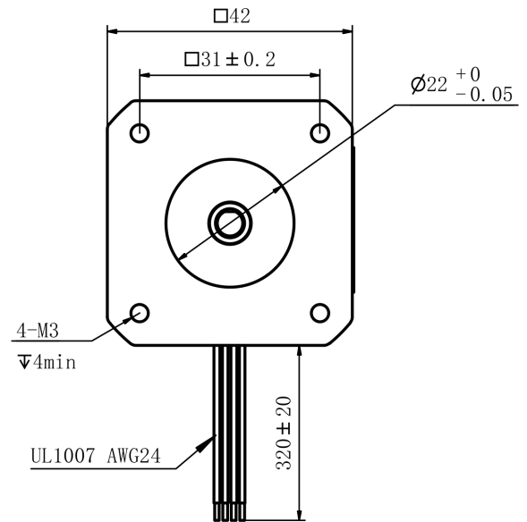
Mechanical View 2
