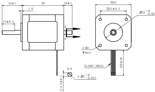
Mechanical View 1
