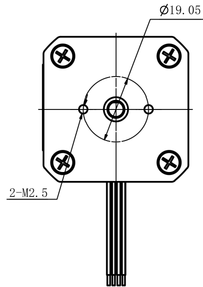
Mechanical View 2
