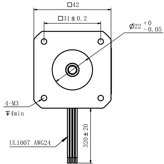
Mechanical View 2
