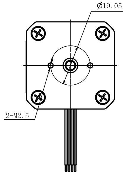
Mechanical View 2
