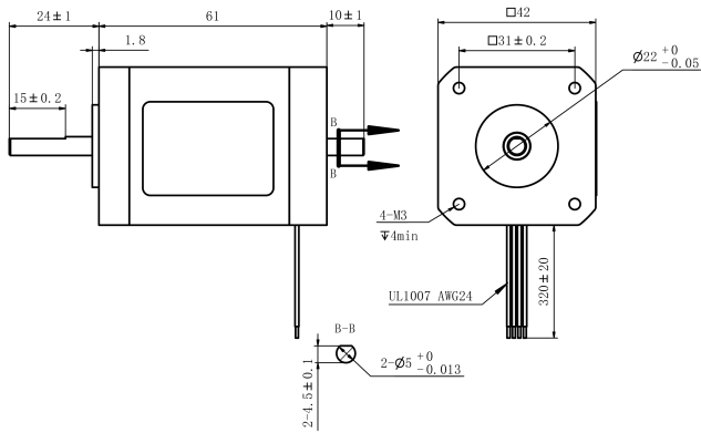
Mechanical View 1
