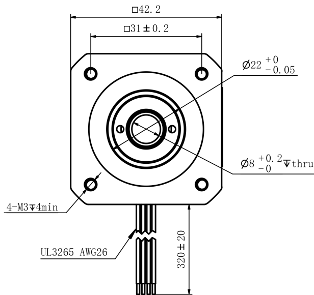
Mechanical View 1
