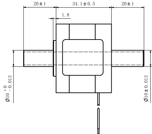
Mechanical View 2
