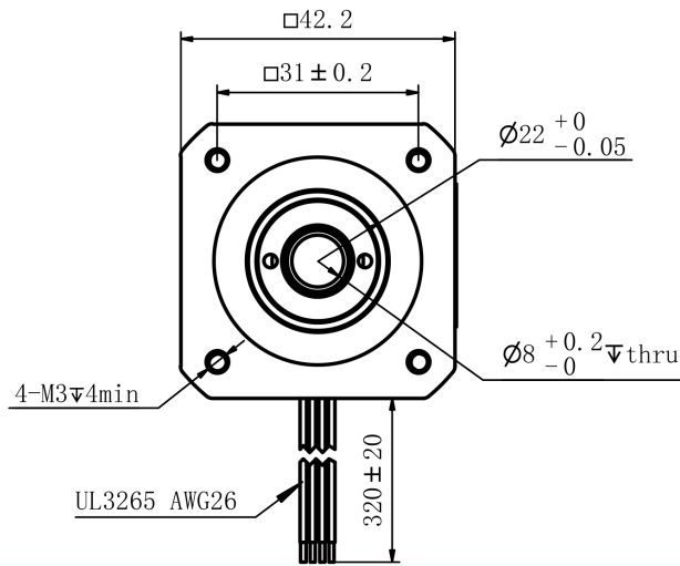
Mechanical View 1
