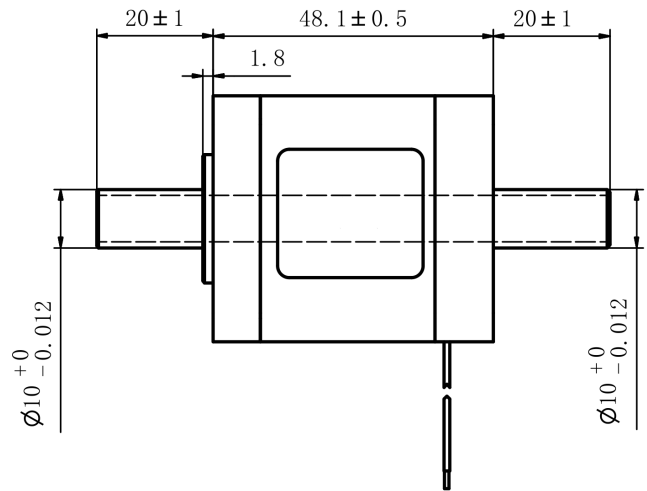
Mechanical View 2
